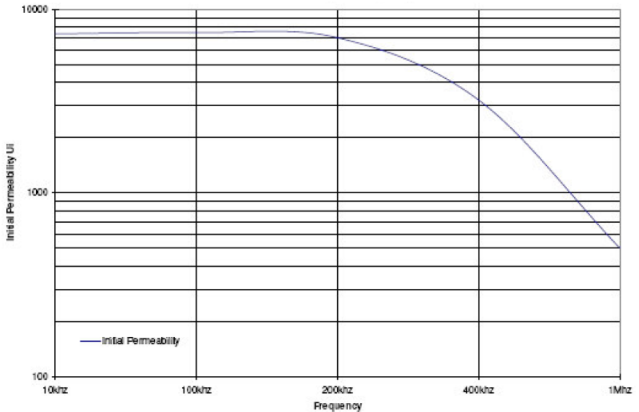
Initial Permeability versus frequency (Measured on T 2512 Toroids)
